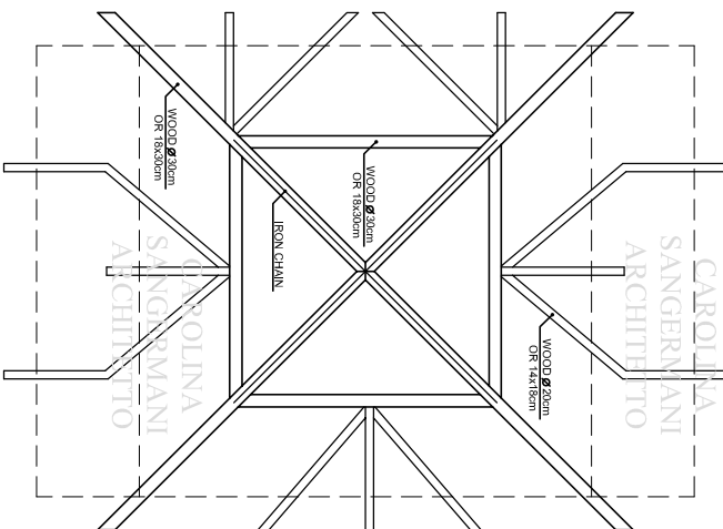
ROOF STRUCTURE OUTLINE
