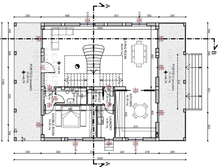
GROUND FLOOR H=270
